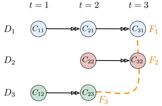
Fig. 1. Example of three dynamic communities tracked over three time steps, featuring continuation, birth, and death community life-cycle events.
