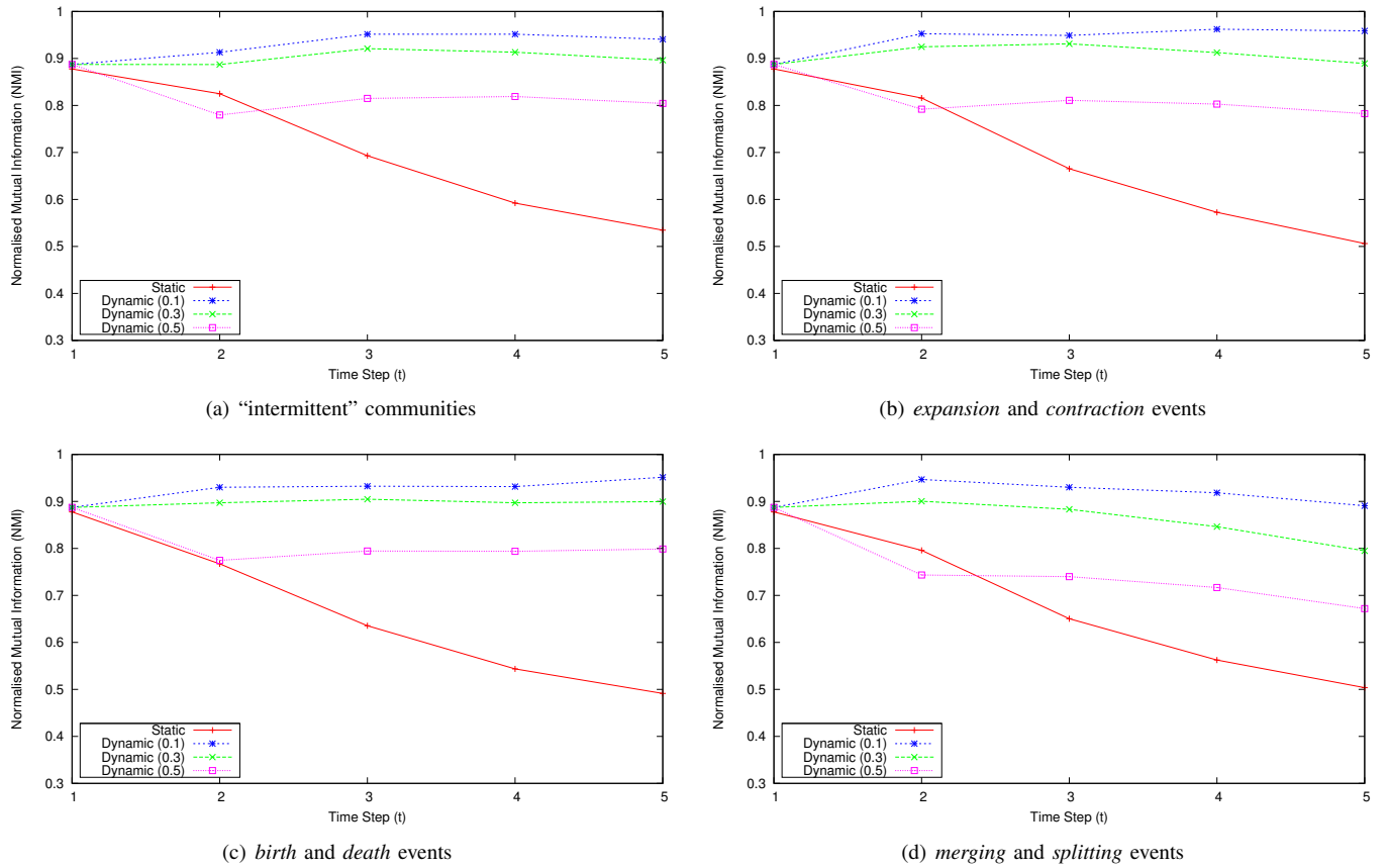
Fig. 6. Performance, in terms of Normalised Mutual Information (NMI), of the proposed dynamic community finding method on four synthetic networks containing different types of embedded community events.
